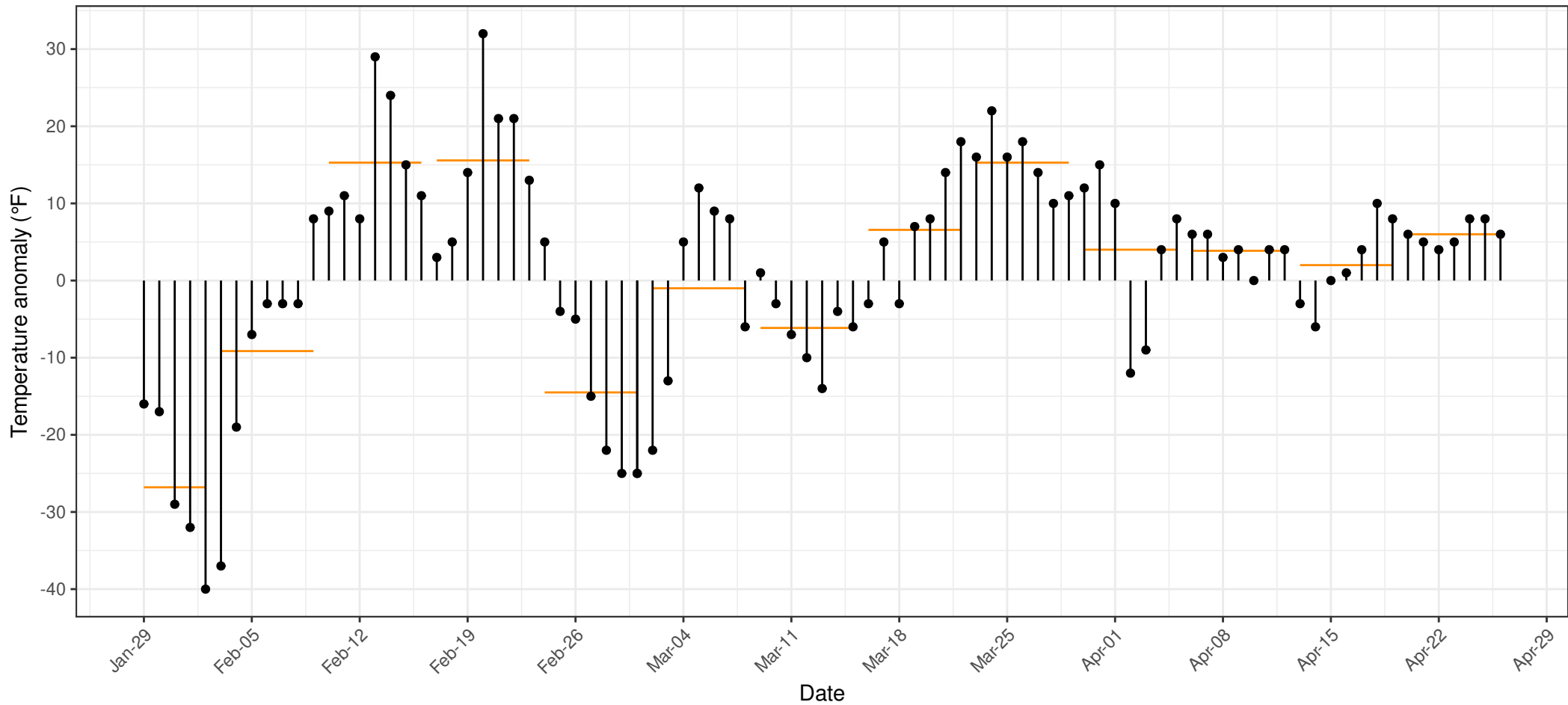
Difference between daily mean temperature and 30-year average, Fairbanks Airport (PAFA) 2024
