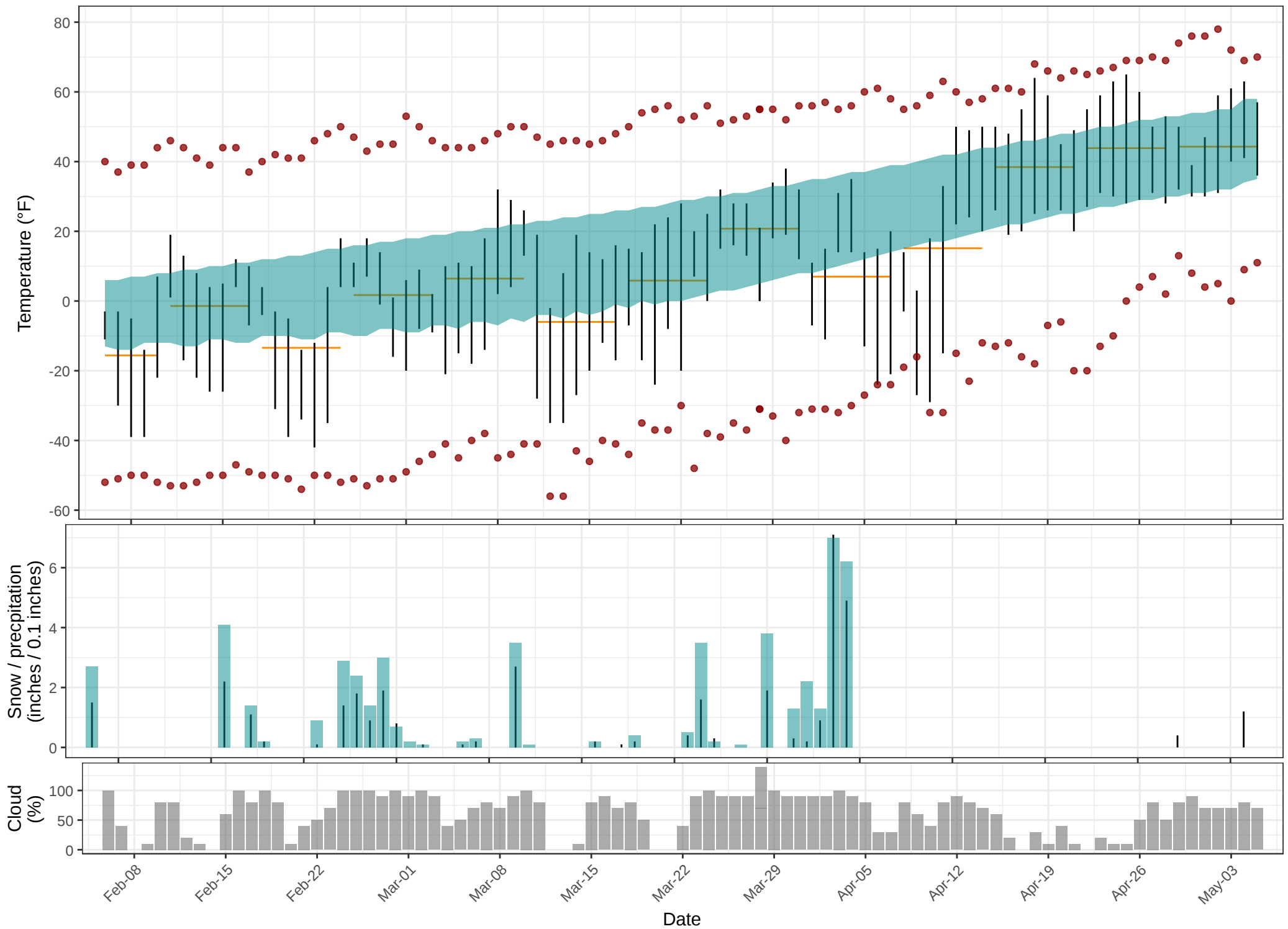
Daily temperature, precipitation and cloud cover, Fairbanks Airport (PAFA) 2021
