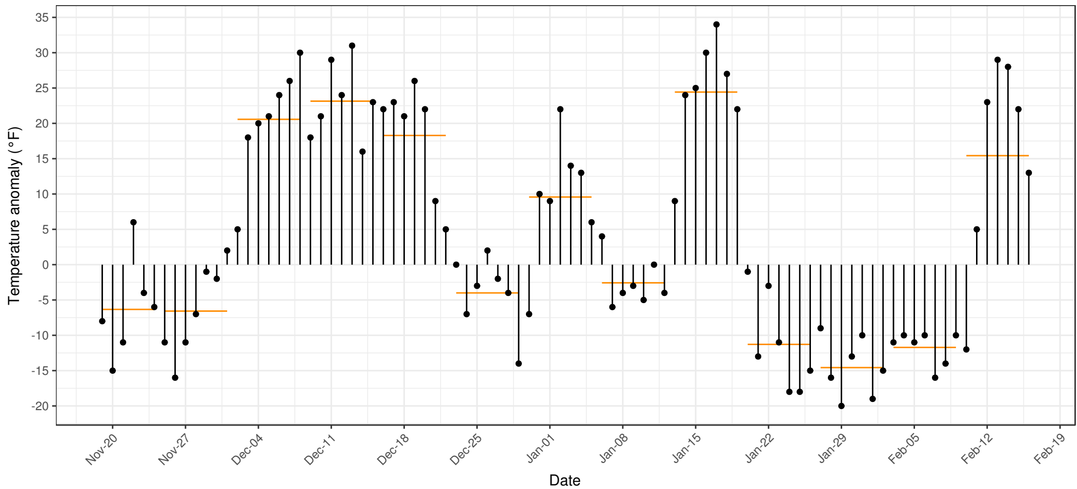
Difference between daily mean temperature and 30-year average, Fairbanks Airport (PAFA) 2017–2018
