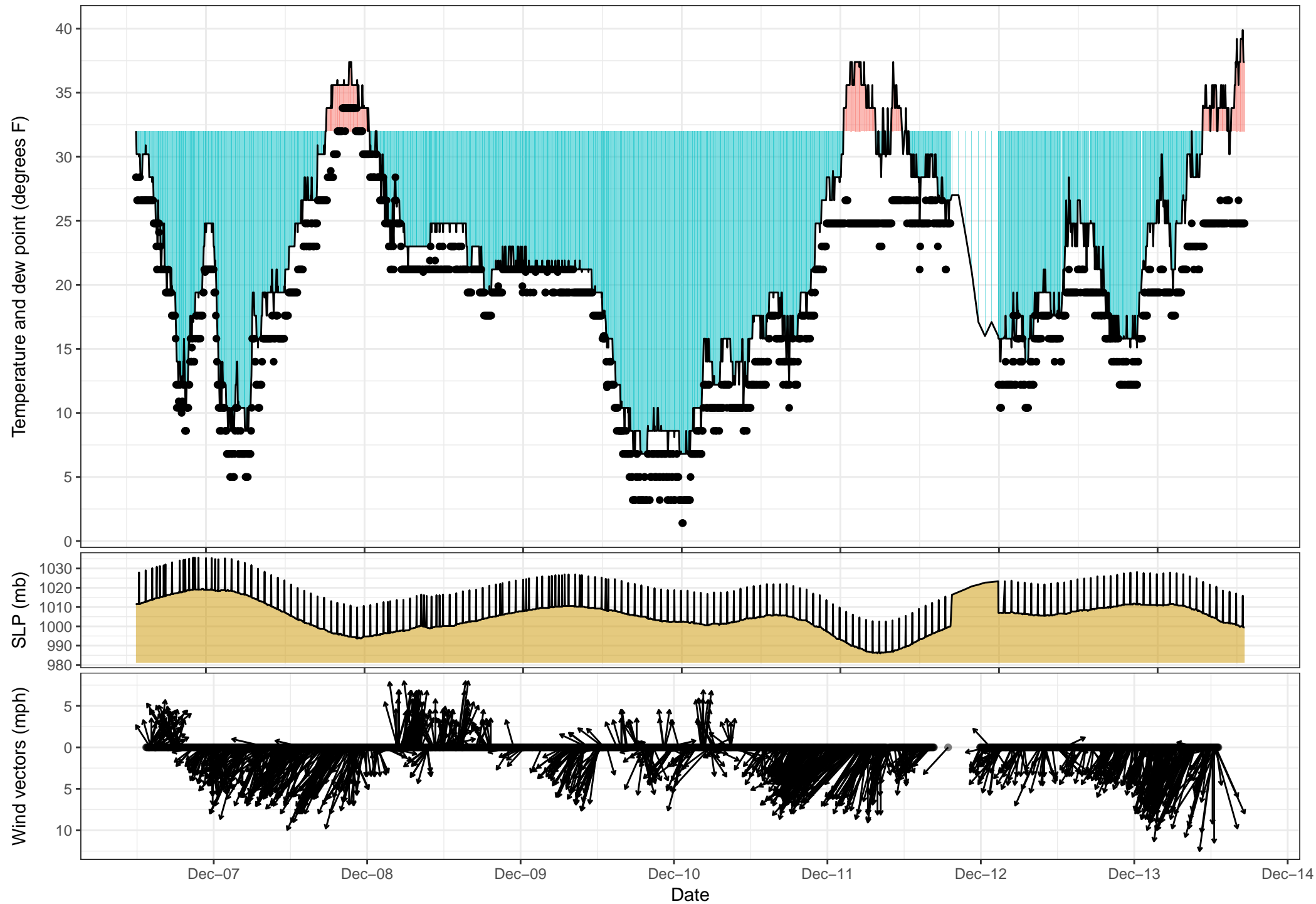
Temperature, dew point, barometric pressure and wind, Fairbanks Airport (PAFA)
